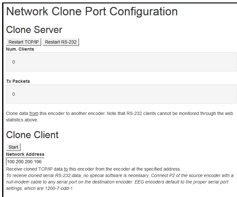
Figure 15: Clone Settings on the Encoder Web Interface
